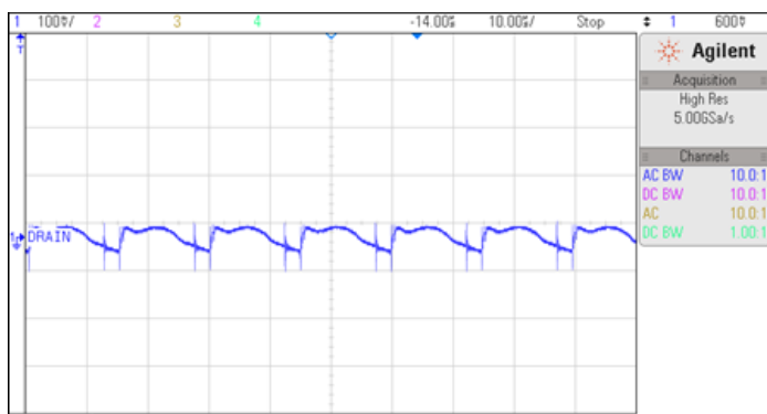
Figure:17 5V Ripple at 230Vac at FL
