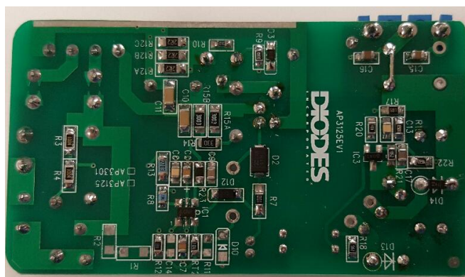
Figure 2: Bottom View
