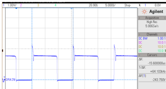
Fig:6 Vds at full load by using DF probe 1:100 at 115V AC
