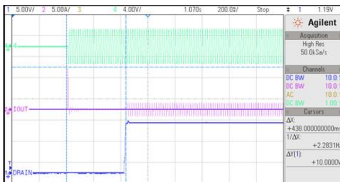
Fig:13 Turn on VAC_in, IAC_in, 12Vo at 230Vac at FL
