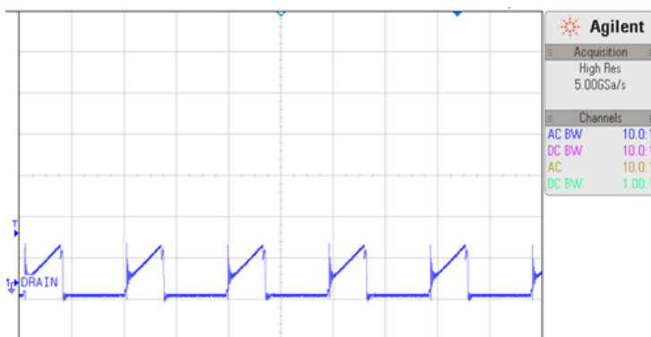
Fig:10 Vcs at 115V ACin at FL
