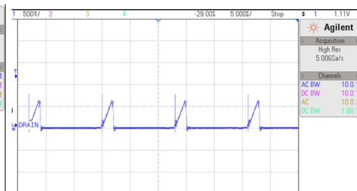
Fig:11 Vcs at 264V ACin at FL
